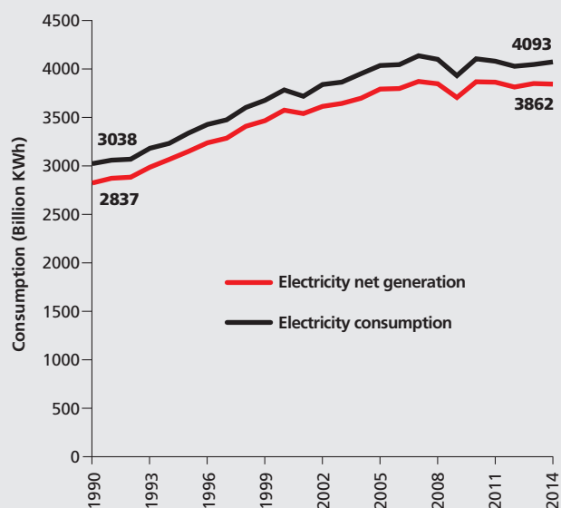
Graph 3.2: Electricity generation and consumption in the US
