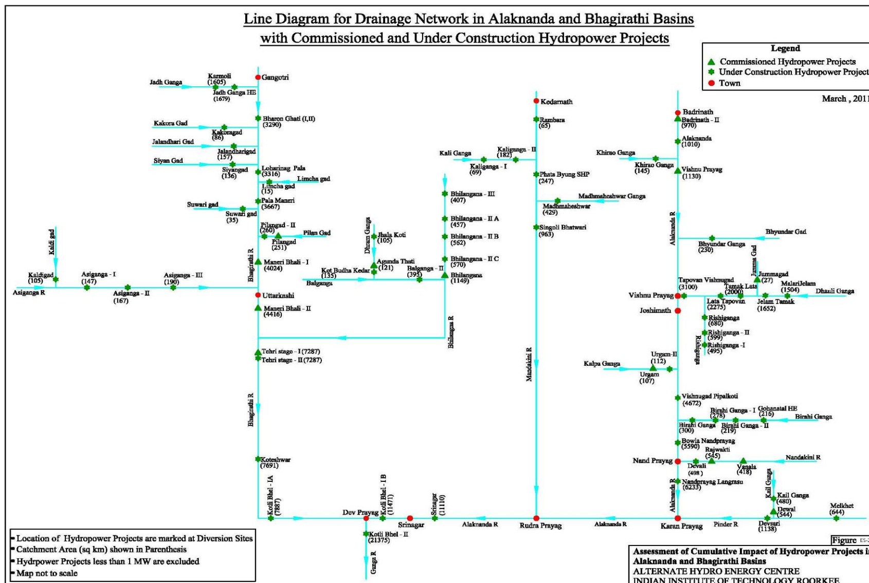
Fig. ES-4: Line Diagram for Drainage Network in Alaknanda and Bhagirathi Basins with hydropower projects
